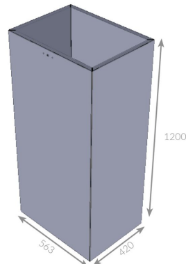
Dreamoc HD3.2 Stand - measurements
